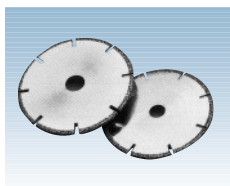
Automatic grooving blade in hardened steel with diamond coated tips for grooving up to 2000 linear metres of safety flooring. AGBL model to fit Leister's Fraesrex grooving machine (N.B. fit with fibre washer at front of blade for correct alignment); AGBM model to fit Mafell's KFU 1000 grooving machine (N.B. fit with fibre washer at back of blade for correct alignment).
