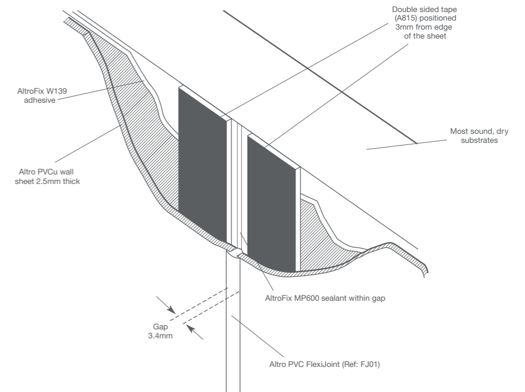
Altro wall sheet to Altro Whiterock FlexiJoint detail
